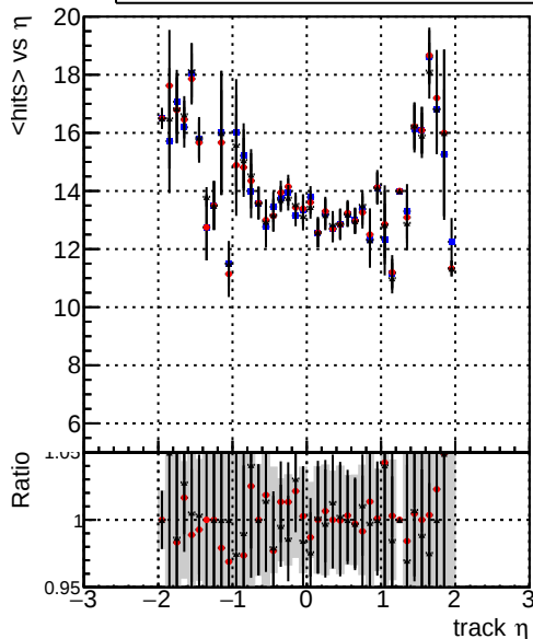
mean hit — DQM_mkFit_TToriginal — DQM_mkFit_TTNEWHS_ALLITERS — DQM_mkFit_TTNEWHSMS_ALLITERS
