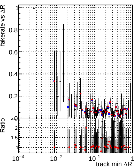
Fake rate vs \Delta R(\text{track, jet}) Legend: DQM_mkFit_TToriginal (blue dots) DQM_mkFit_TTNEWHS_ALLITERS (red dots) DQM_mkFit_TTNEWHSMS_ALLITERS (black dots with error bars)
