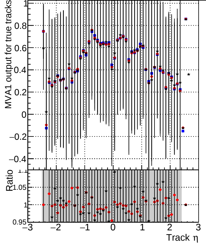
MVA1 of associated tracks (recoToSim) vs. track \eta Legend: DQM_mkFit_TToriginal (blue squares) DQM_mkFit_TTNEWHWS_ALLITERS (red circles) DQM_mkFit_TTNEWHSMS_ALLITERS (black stars)
