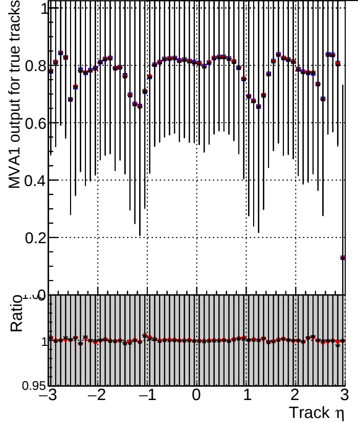
MVA1 of associated tracks (recoToSim) vs. track \eta Legend: ■ DQM_mkFit_TToriginal ● DQM_mkFit_TTNEWHWS_ALLITERS ▲ DQM_mkFit_TTNEWHWSMS_ALLITERS
