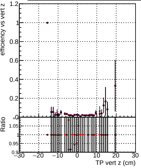
Efficiency vs vert z Legend: DQM_mkFit_TToriginal DQM_mkFit_TTNEWSMS_ALLITERS DQM_mkFit_TTNEWSMS_ALLITERS
