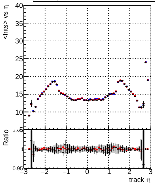
DQM_mkFit_TToriginal DQM_mkFit_TTNEWHS_ALLITERS DQM_mkFit_TTNEWHSMS_ALLITERS mean hit
