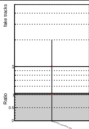
N of fake track vs. \chi^2
