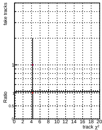
N of fake track vs. \chi^2
