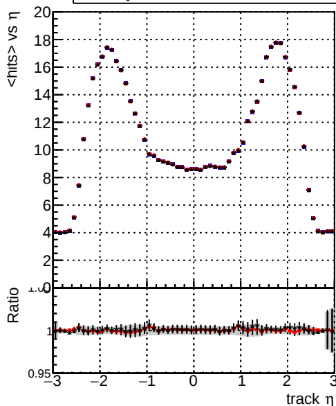
DQM_mkFit_TToriginal DQM_mkFit_TTNEWHS_ALLITERS DQM_mkFit_TTNEWHSMS_ALLITERS mean hit
