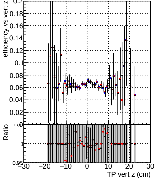
Efficiency vs. sim PV z —●— DQM_mkFit_TToriginal —●— DQM_mkFit_TTNEUHS_ALLITERS —●— DQM_mkFit_TTNEUHSMS_ALLITERS
