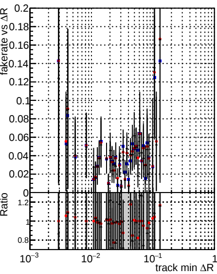
Fake rate vs \Delta R(\text{track, jet}) Legend: DQM_mkFit_TToriginal (black line with dots) DQM_mkFit_TTNEWHS_ALLITERS (red line with dots) DQM_mkFit_TTNEWHSMS_ALLITERS (blue line with dots)
