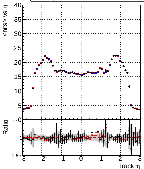
mean hit — DQM_mkFit_TToriginal — DQM_mkFit_TTNEUHS_ALLITERS — DQM_mkFit_TTNEUHSMS_ALLITERS
