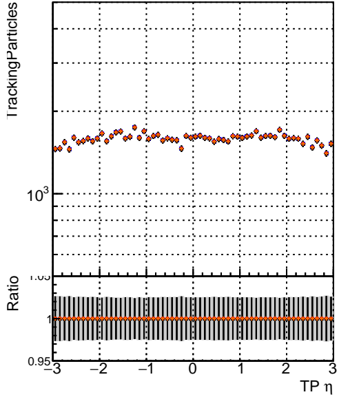
N of simulated tracks vs \eta Legend: DQM_mkFit TT original DQM_mkFit TT pL DQM_mkFit TT pLW DQM_mkFit TT pLW IMP
