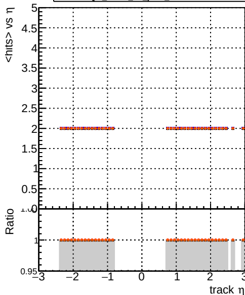
DQM_mkFit_TToriginal DQM_mkFit_TT_pL DQM_mkFit_TT_pLW DQM_mkFit_TT_pLW IMP
