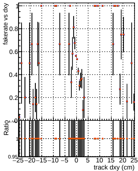
Fake rate vs d —•— DGM mkt Fit T original —•— DGM mkt Fit T BEW IMP
