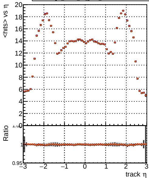
mean hit DQM_mkFit_TToriginal DQM_mkFit_TT_pL DQM_mkFit_TT_pLW DQM_mkFit_TT_pLW IMP
