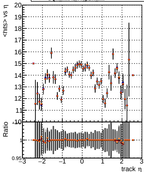
mean hits vs \eta DQM_mkFit_TToriginal DQM_mkFit_TT_pL DQM_mkFit_TT_pLW DQM_mkFit_TT_pLW IMP
