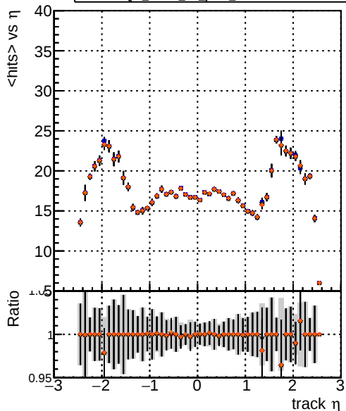
Legend for mean hits vs \eta : DOM_mkFit_TToriginal (blue line with circles) DOM_mkFit_TT_pL (red line with circles) DOM_mkFit_TT_pLW (black line with circles) DOM_mkFit_TT_pLW IMP (orange line with circles)
