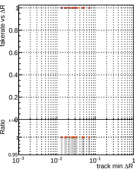
Fake rate vs \Delta R(\text{track, jet}) Legend: DOM mkFit TToriginal DOM mkFit TTBLW DOM mkFit TTBLW IMP
