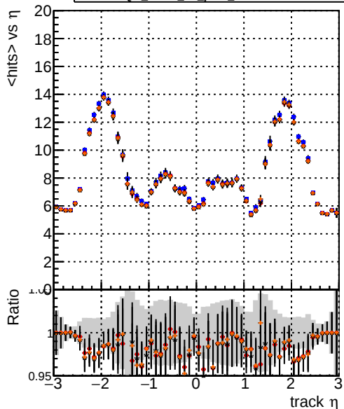
DQM_mkFit_TToriginal DQM_mkFit_TT_pL DQM_mkFit_TT_pLW DQM_mkFit_TT_pLW IMP mean hit
