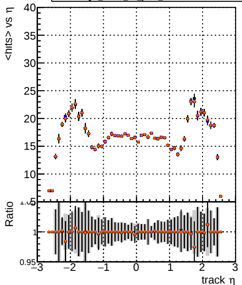
DQM_mkFit_TToriginal DQM_mkFit_TT_pL DQM_mkFit_TT_pLW DQM_mkFit_TT_pLW IMP
