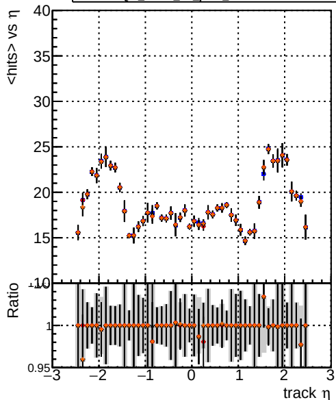
Legend: DQM_mkFit TT original (blue line), DQM_mkFit TT pL (red line), DQM_mkFit TT pLW (black line), DQM_mkFit TT pLW IMP (orange line) mean hit
