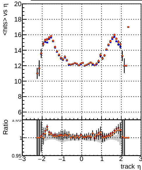
DQM_mkFit_TToriginal DQM_mkFit_TT_pL DQM_mkFit_TT_pLW DQM_mkFit_TT_pLW IMP mean hit
