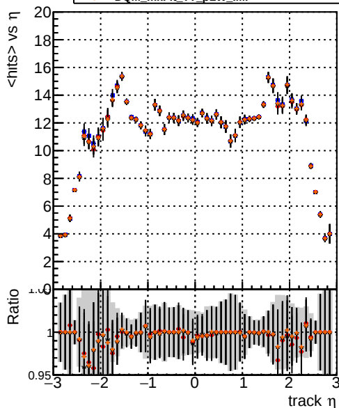
DQM_mkFit_TToriginal DQM_mkFit_TT_pL DQM_mkFit_TT_pLW DQM_mkFit_TT_pLW IMP mean hits
