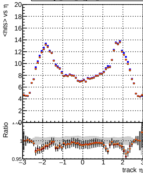
Legend: DQM_mkFit TT original (blue line), DQM_mkFit TT pL (red line), DQM_mkFit TT pLW (black line), DQM_mkFit TT pLW IMP (orange line) mean hit
