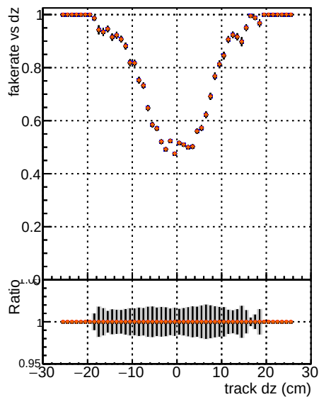
Fake rate vs d Legend: DOM, mkt, T, Original, DOM, mkt, T, BEW, 1H
