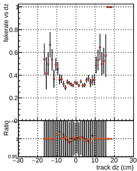
Legend: DSM mkFit T Original DSM mkFit T BEW 1H
