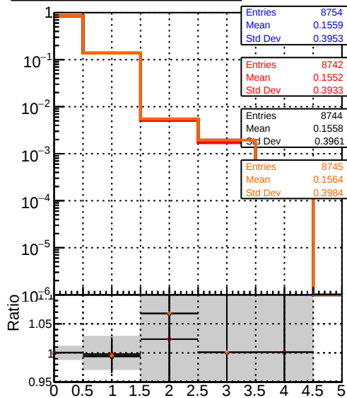
Legend: DQM_mkFit_TToriginal (blue line) DQM_mkFit_TT_pL (red line) DQM_mkFit_TT_pLW (black line) DQM_mkFit_TT_pLW_1H (orange line) mean hit
