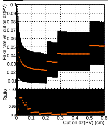
Fake rate
