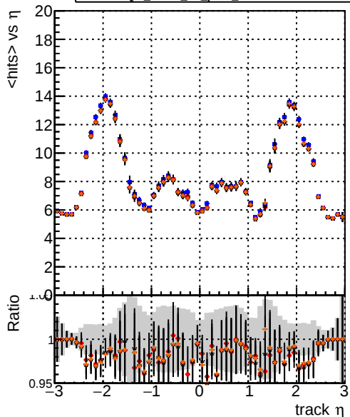
Legend: DOM_mkFit_TToriginal DOM_mkFit_TT_pL DOM_mkFit_TT_pLW DOM_mkFit_TT_pLW_1H mean hit
