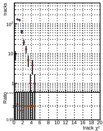
N of reco track vs. \chi^2 BSM mkFit BSM mkFit + 1H Original
