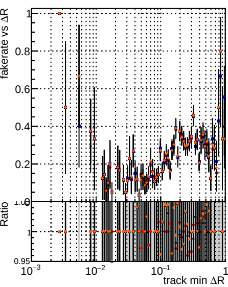
Fake rate vs \Delta R(\text{track, jet}) Series Line Style Marker DOM Solid Black mktFit Dashed Blue original Dotted Red BLW Solid Orange 1H Solid Grey
