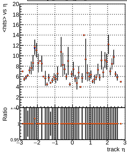
DQM_mkFit_TToriginal DQM_mkFit_TT_pL DQM_mkFit_TT_pLW DQM_mkFit_TT_pLW_1H mean hit
