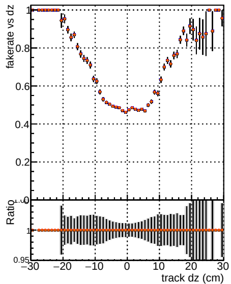
Legend for Fake rate vs d: DSM mkFit T Original DSM mkFit T BEW 1H
