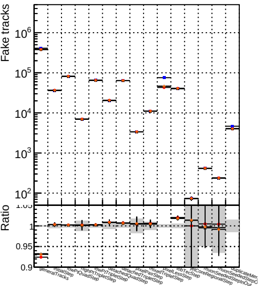
Number Legend —▲— DQM_mkFit_TT_pLW —+— DQM_mkFit_TT_pLW_1H
