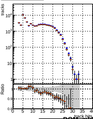
N of reco track vs track hits
