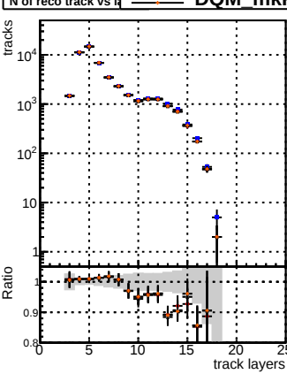
N of reco track vs track layers
