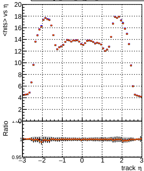
mean hit DOM_mkFit_TToriginal DOM_mkFit_TT_pL DOM_mkFit_TT_pLW DOM_mkFit_TT_pLW_1H
