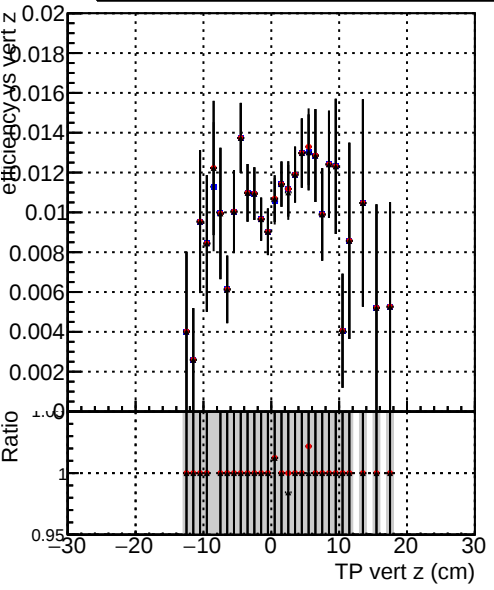
Efficiency vs TP vert z (cm) Legend: DQM_mkFit_TToriginal (blue star) DQM_mkFit_TT_pL (red star) DQM_mkFit_TT_pLW (black star)
