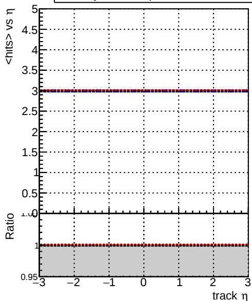
mean hits DQM_mkFit_TToriginal DQM_mkFit_TT_pL DQM_mkFit_TT_pLW
