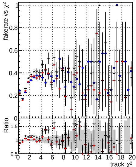
Fake rate vs. —●— DOM mkFit TToriginal —●— DOM mkFit TT PLW
