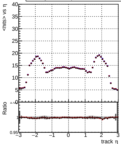
DQM_mkFit_TToriginal DQM_mkFit_TT_pL DQM_mkFit_TT_pLW mean hit
