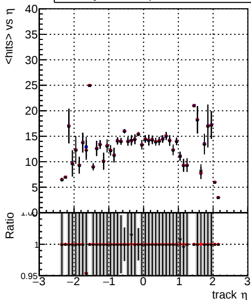
mean hit — DQM_mkFit_TToriginal — DQM_mkFit_TT_pL — DQM_mkFit_TT_pLW
