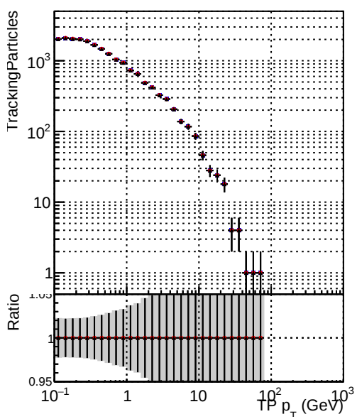
Legend: DQM_mkFit_TToriginal (blue), DQM_mkFit_TT_pL (red), DQM_mkFit_TT_pLW (black)
