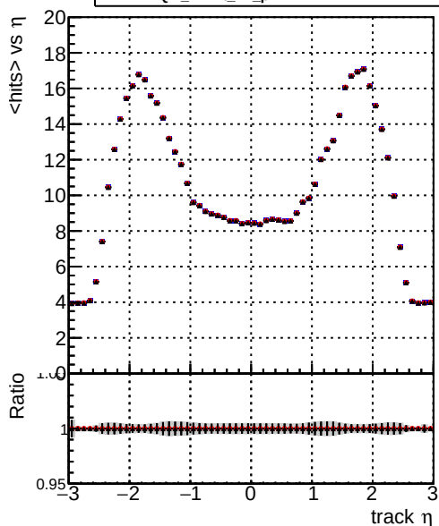
mean hits — DQM_mkFit_TToriginal — DQM_mkFit_TT_pL — DQM_mkFit_TT_pLW
