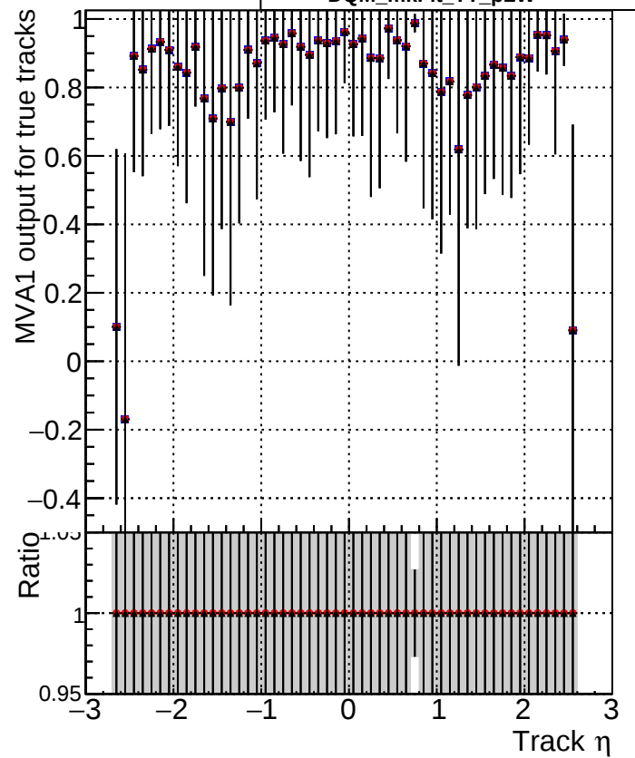
MVA1 of associated tracks (recoToSim) vs. track \eta Legend: DQM_mkFit_TToriginal (blue square) DQM_mkFit_TT_pL (red circle) DQM_mkFit_TT_pLW (black triangle)
