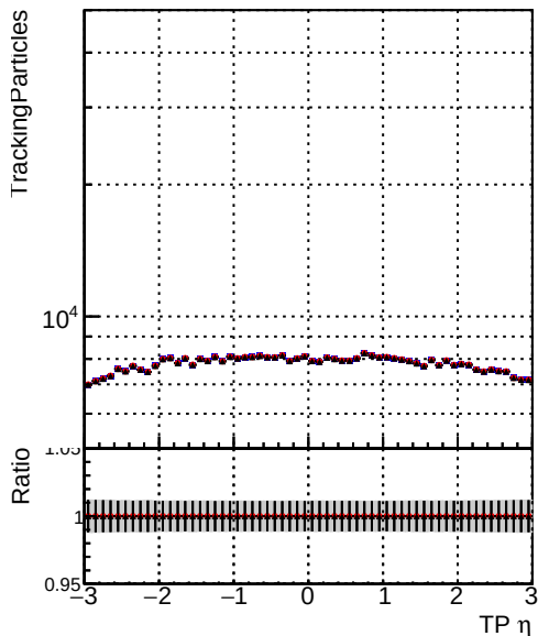
Legend: DQM_mkFit_TToriginal (blue circles) DQM_mkFit_TT_pL (red circles) DQM_mkFit_TT_pLW (black circles)
