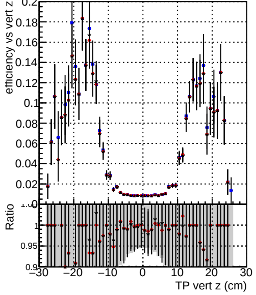
Efficiency vs. TP vert z (cm) —●— DQM_mkFit_TToriginal —●— DQM_mkFit_TT_pL —●— DQM_mkFit_TT_pLW
