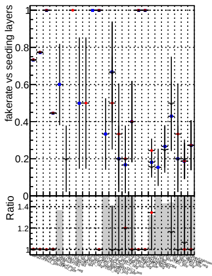
Fake rate vs. BQM mkFit TToriginal BQM mkFit TT BQM mkFit TT BQM mkFit TT BQM mkFit TT
