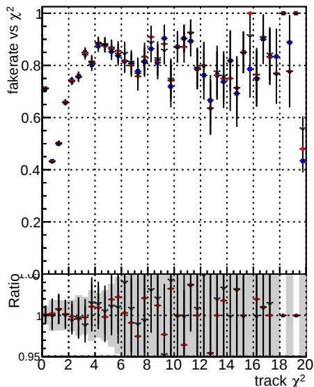
Fake rate vs. BQM mkFit TToriginal BQM mkFit TT BQM mkFit TT BQM mkFit TT BQM mkFit TT
