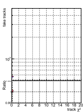
N of fake track vs normalized \chi^2
