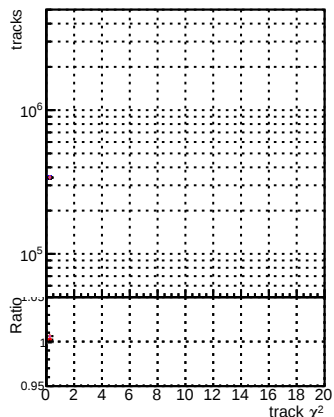
N of reco track vs. \chi^2 DOM mFit TT new study v4
